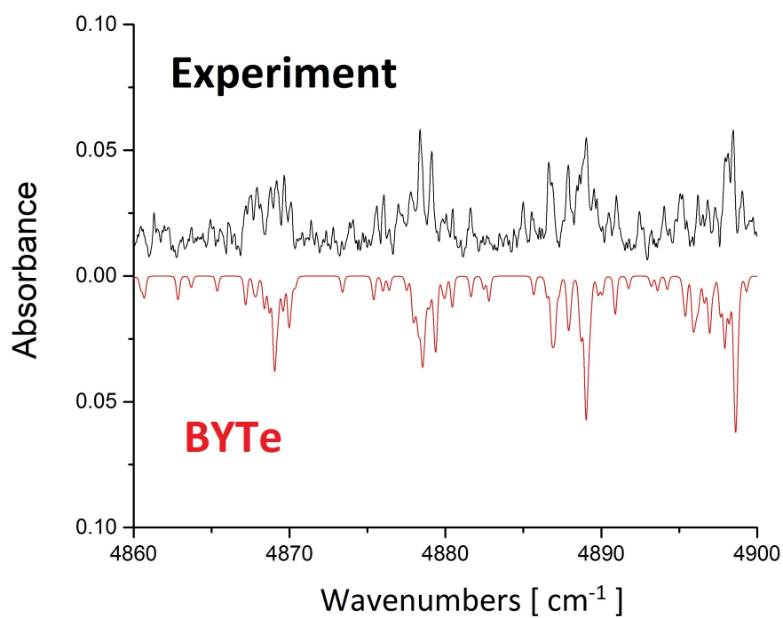
Figure 4: Comparison between experimental (upper) and calculated (BYTe, lower) absorption spectra at 1027 °C for the range 4860 - 4900 cm -1 .
