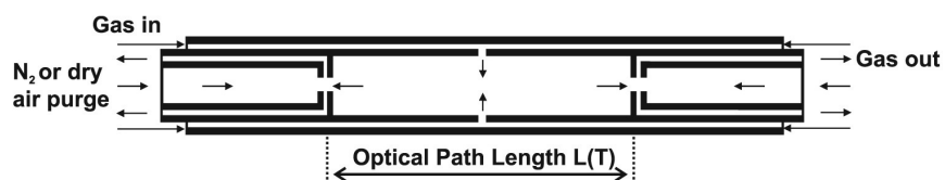
Figure 1: High temperature ceramic gas flow cell (c-HGC) used in the experiments. Black arrows indicate flow direction. Reproduced from [34].
