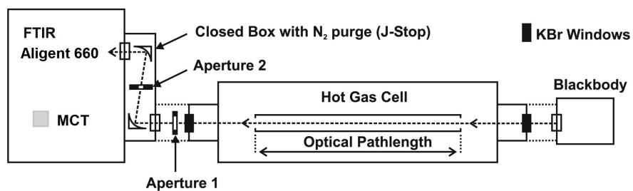
Figure 2: Experimental setup for the high-resolution measurements of \text{NH}_3 at high temperatures. Adapted from [34].
