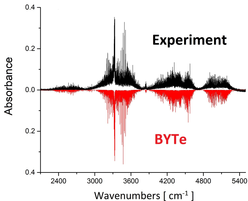
Figure 3: Comparison between experimental (upper) and calculated (BYTe, lower) absorption spectra at 500 °C for the range 2100 - 5500 \text{cm}^{-1} .
